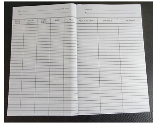
Level Book
